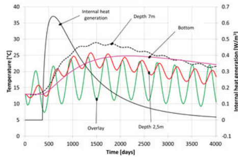
Fig. 5 Trend of the temperature inside of the landfill
