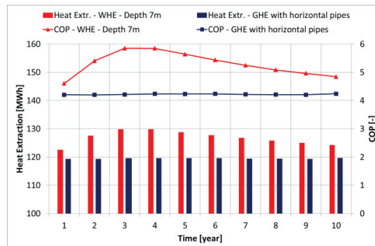
Fig. 8 Annual COP values and heat extraction over ten years of operation at 45°C on the condenser side
