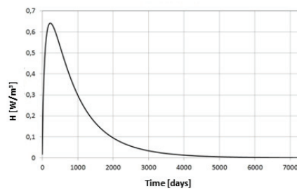
Fig. 3. Internal heat production of the waste
