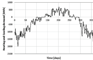
Fig 4. Heating and cooling load profile of the users for the case study
