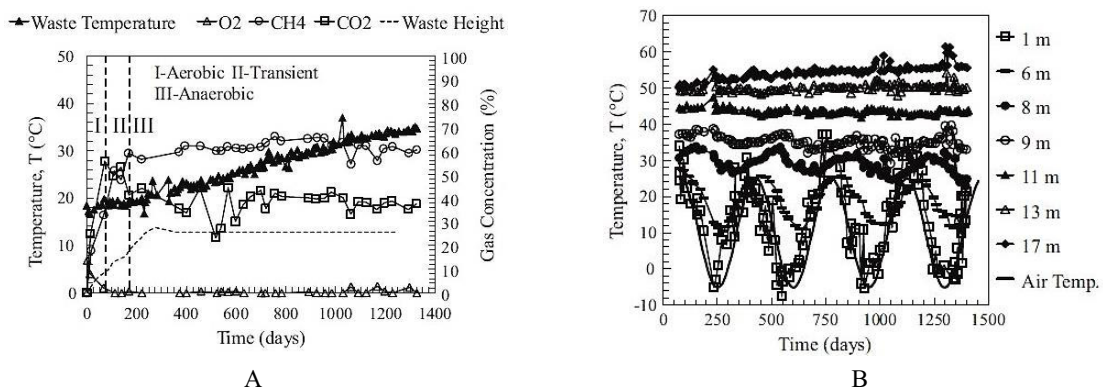
Fig. 1. Example of temperature raised in a landfill of MSW [3]: A) Identification of three stages of the degradation of the solid waste; B) Trend of the temperature inside of the landfill for different depth
