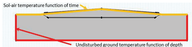
Fig. 2. Section of the landfill
