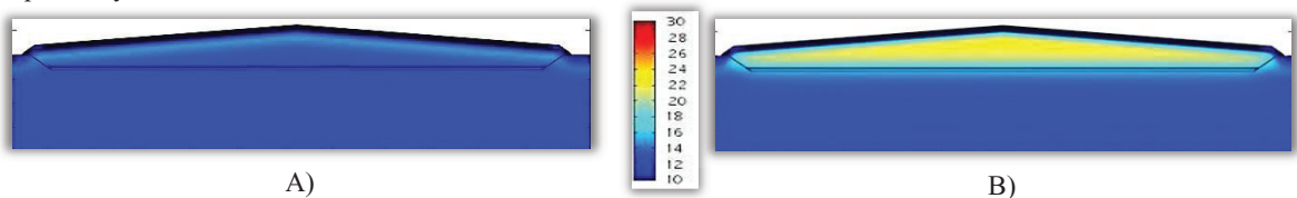
A) B) Fig. 7. Temperature in °C of the landfill during the 20th of December: A) without the internal heat generation, B) with the internal heat generation
