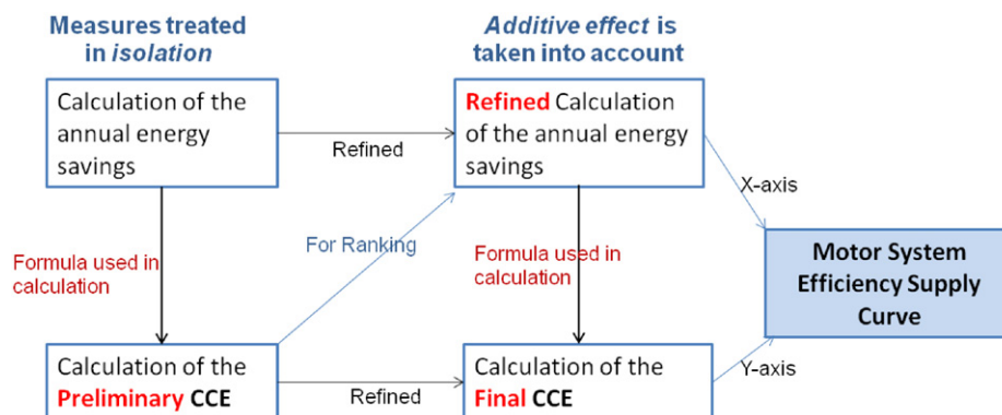
Fig. 1. Schematic of calculation process for the construction of motor systems efficiency supply curves.
