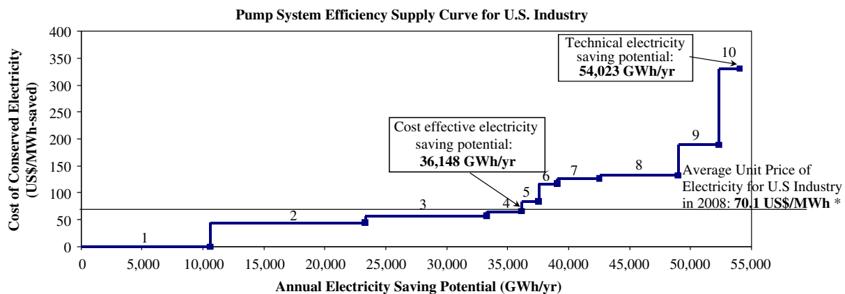
Fig. 2. US Pumping System Efficiency Supply Curve. Note: This supply curve is intended to provide an indicator of the relative cost-effectiveness of system energy efficiency measures at the national level. The cost-effectiveness of individual measures will vary based on site-specific conditions.
