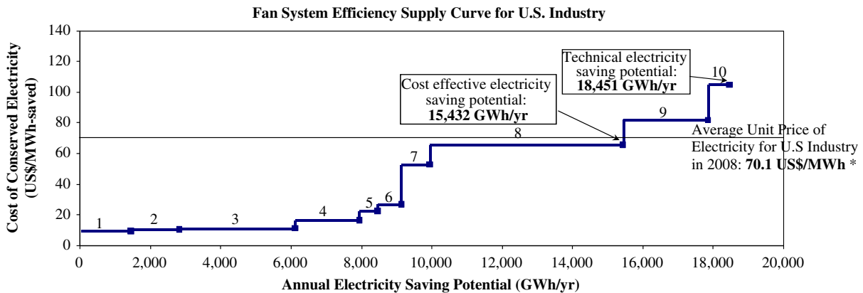
Fig. 4. US Fan System Efficiency Supply Curve. Note: This supply curve is intended to provide an indicator of the relative cost-effectiveness of system energy efficiency measures at the national level. The cost-effectiveness of individual measures will vary based on site-specific conditions.
