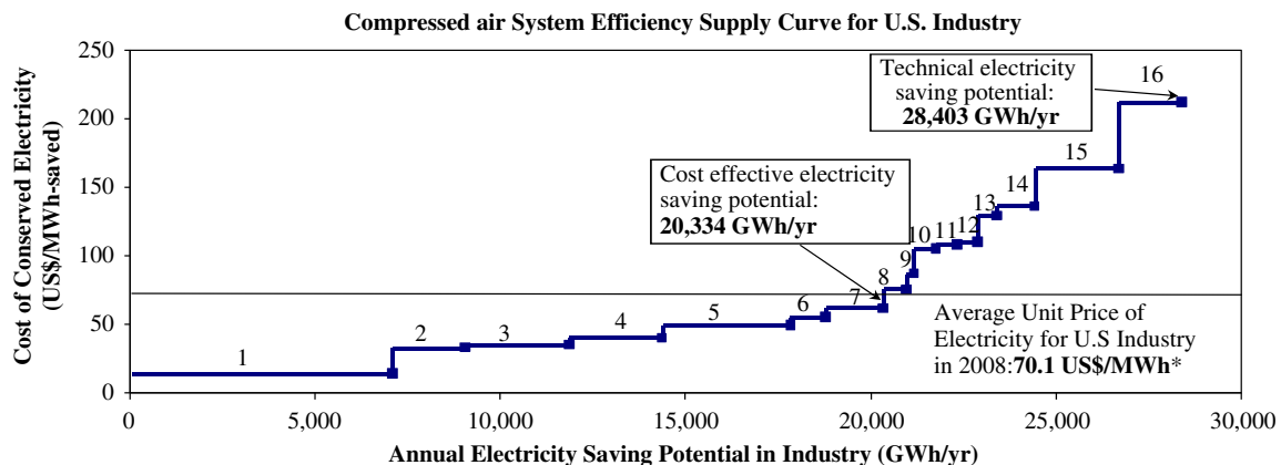
Fig. 3. US Compressed Air System Efficiency Supply Curve. Note: this supply curve is intended to provide an indicator of the relative cost-effectiveness of system energy efficiency measures at the national level. The cost-effectiveness of individual measures will vary based on site-specific conditions.
